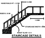
STAIRCASE DETAILS
