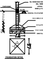
FOUNDATION DET
