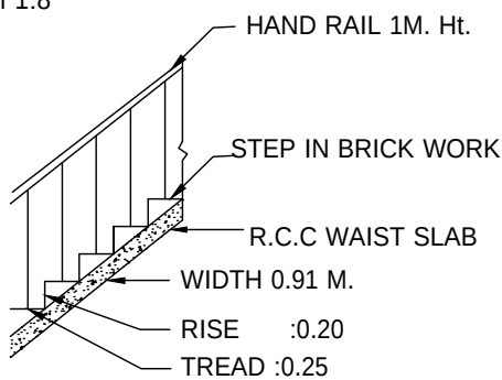
STAIR DETAIL
