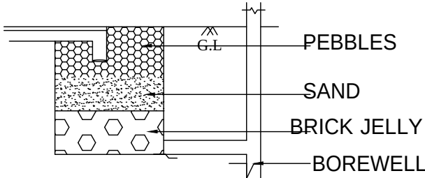
RAINWATER FILTRATION
