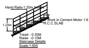
STAIRCASE DETAILS Scale:1:500
