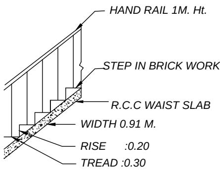
STAIR DETAIL
