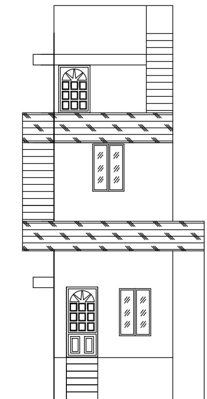
FRONT ELEVATION
