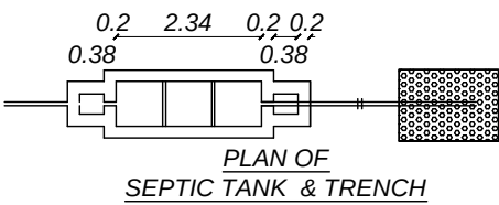
PLAN OF SEPTIC TANK & TRENCH
