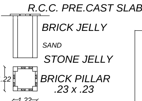
PLAN & SECTION OF RAIN WATER COLLECTION WELL
