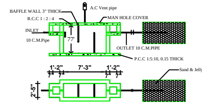
Septic tank and trench
