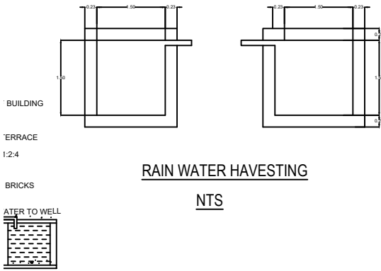
RAIN WATER HARVESTING NTS
