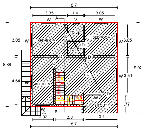
GROND FLOOR PLAN
