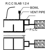
WALL AND TRENCH NTS
