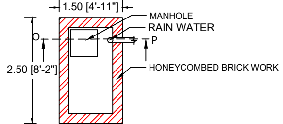
PLAN RAIN WATER HARVESTING
