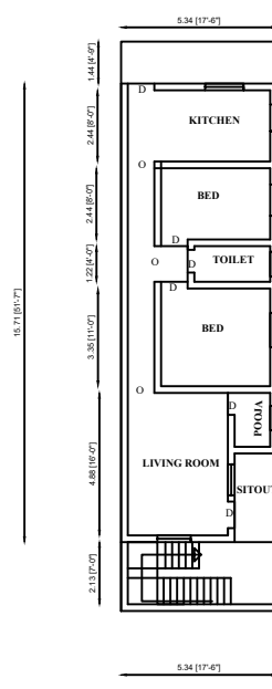
EX .GROUND FLOOR PLAN
