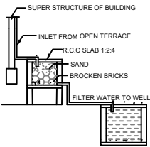
ILS OF FILTER BED & WELL NTS
