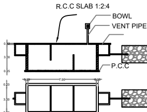
SEPTIC TANK AND TRENCH NTS
