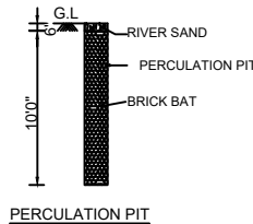
PERCOLATION PIT
