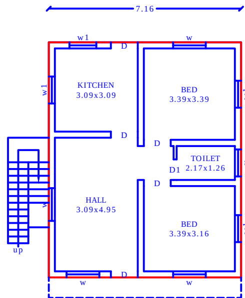
PLAN
