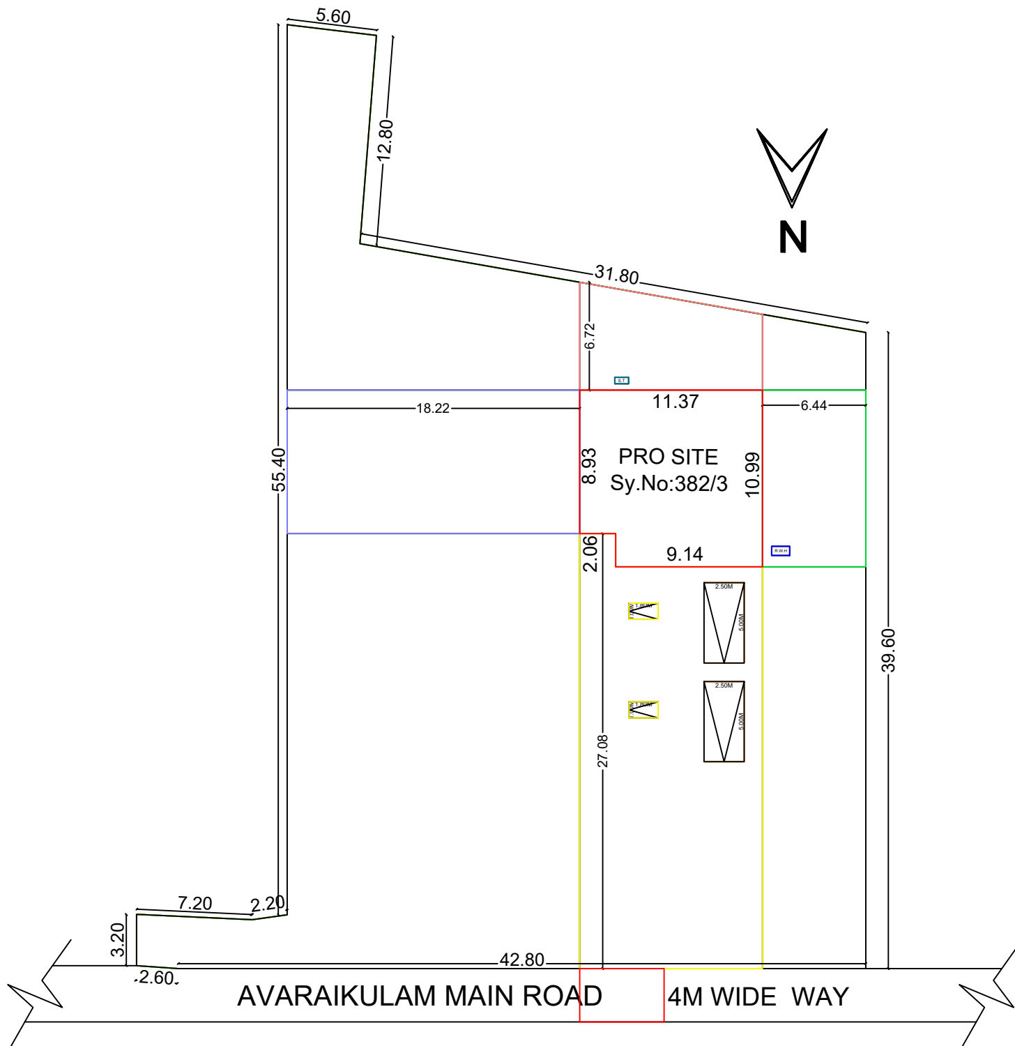
SITE PLAN
