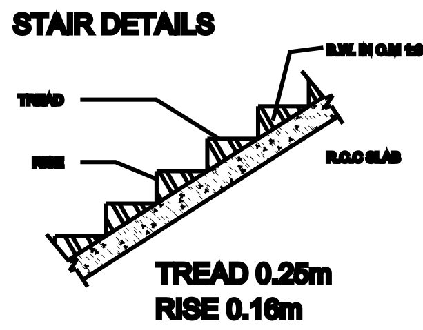
STAIR CASE
