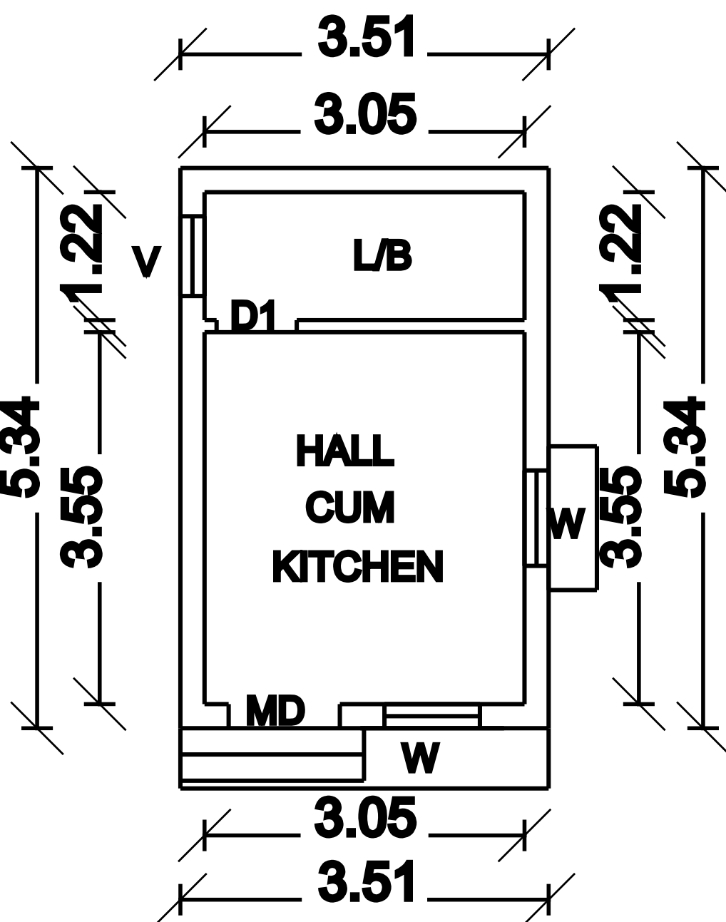
GROUND FLOOR
