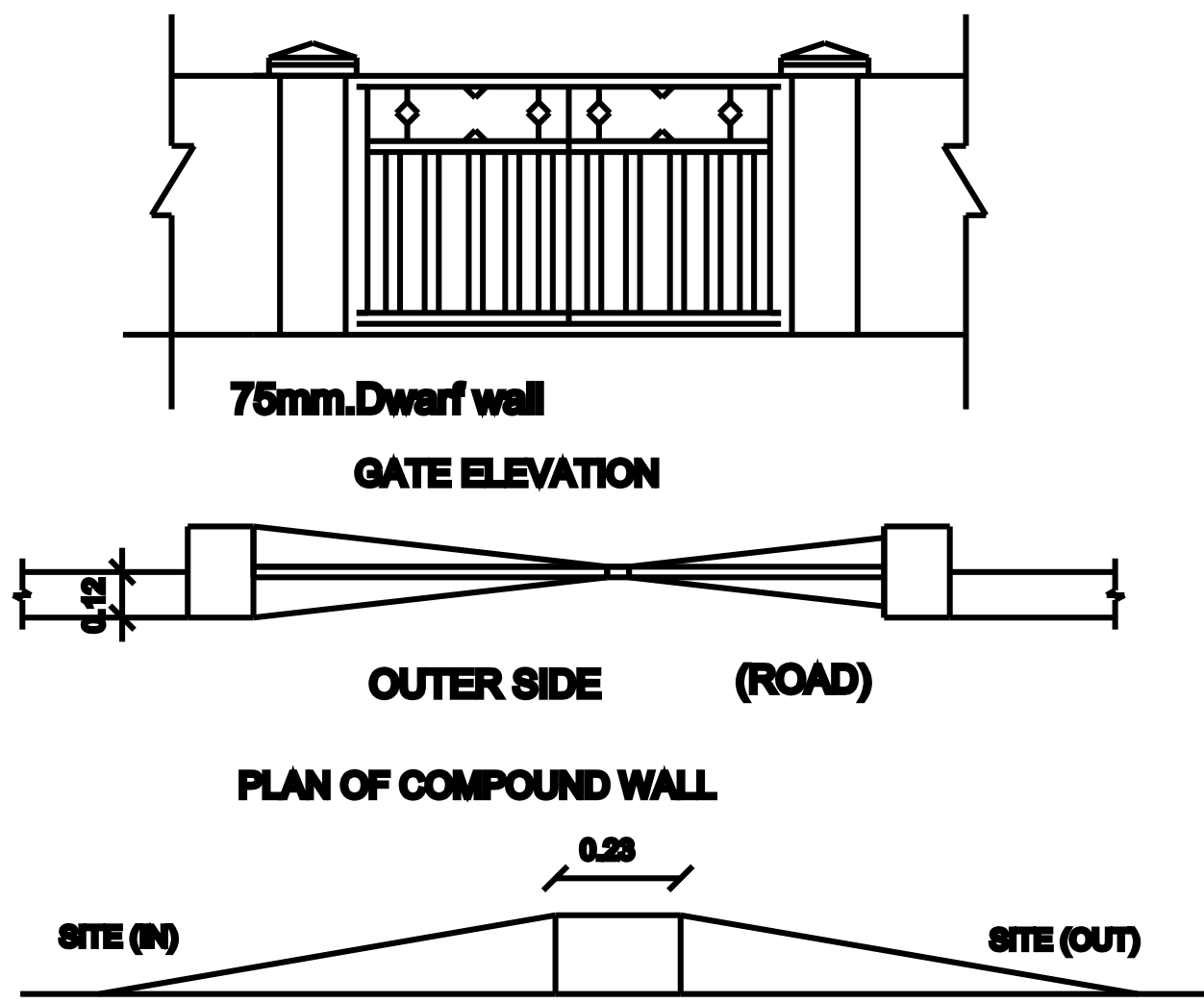
MAIN GATE DETAIL
