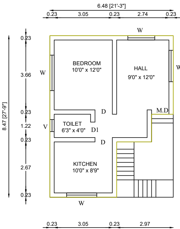
LOOR PLAN
