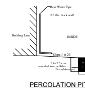
PERCOLATION PI
