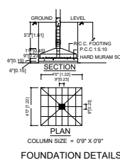
FOUNDATION DETAILS
