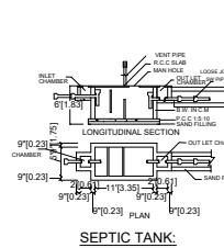
SEPTIC TANK
