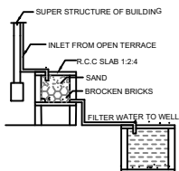
DETAILS OF FILTER BED & WELL
