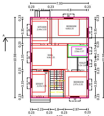
G.F. PLAN
