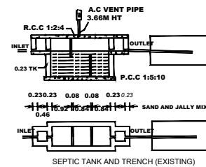
SEPTIC TANK AND TRENCH (EXISTING)
