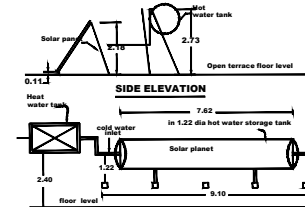
SOLAR WATER HEATER PLANT
