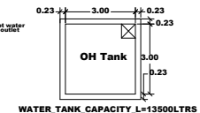
WATER TANK CAPACITY L=13500LTRS
