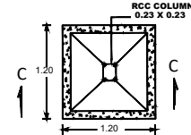
DETAILS OF COLUMN PLAN
