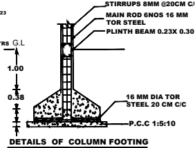
DETAILS OF COLUMN FOOTING
