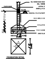
FOUNDATION DETAIL
