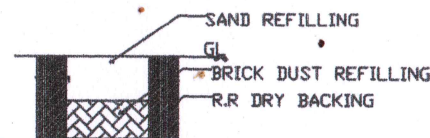
DETAILS OF RAIN WATER HARVESTING
