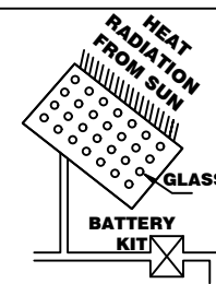
SOLAR SYSTEM
