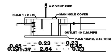
SEPTIC TANK & TRENCH
