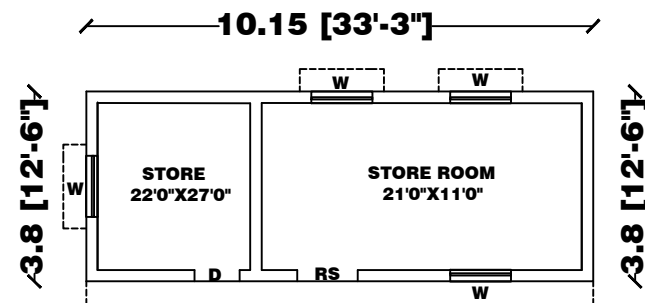
PLAN-1
