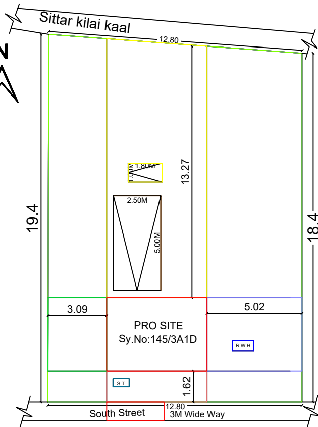
SITE PLAN
