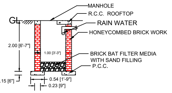
SECTION ON O - P
