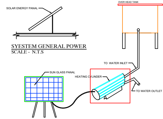
SOLAR WATER HEATING SYSTEM SCALE - N.T.S
