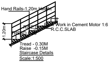
Staircase Details Scale:1:500
