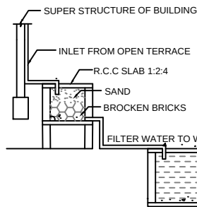
DETAILS OF FILTER BED & WELL
