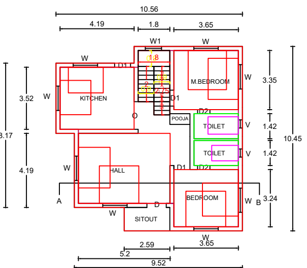
GROND FLOOR PLAN
