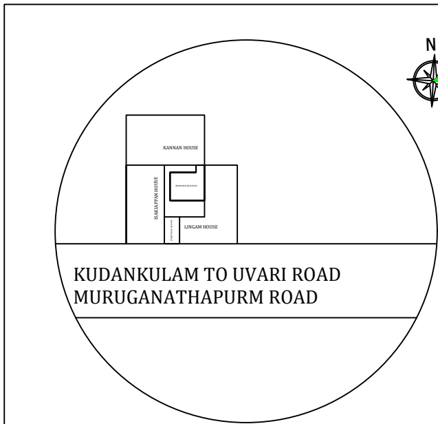
KEY PLAN 1:500
