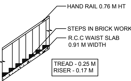
STEP DETAILS
