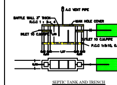
Septic Tank
