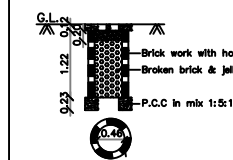
PERCOLATION PIT FOR 30 Sq. m. (Scale: - 1:50)
