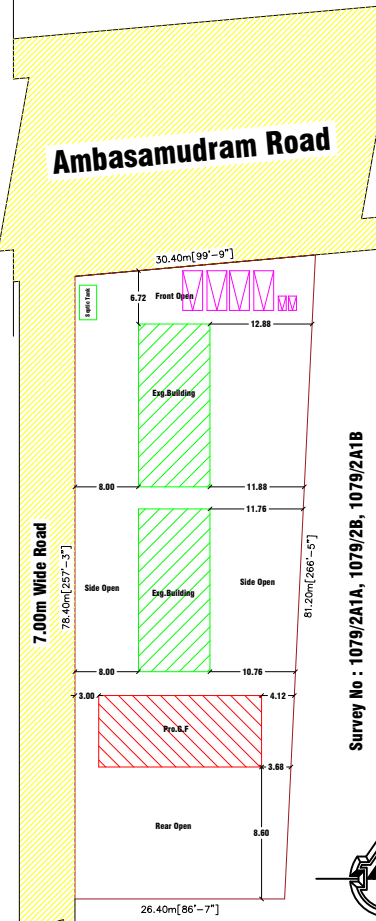
Topo Plan (Not to Scale)
