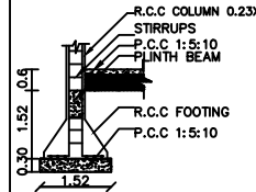
COLOUMN DETAILS
