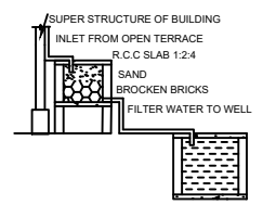
RAINWATER HARVESTING
