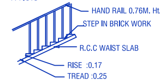
STAIR CASE DETAIL
