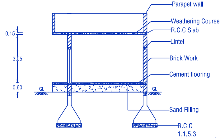
CROSS SECTION ON 'AB'
