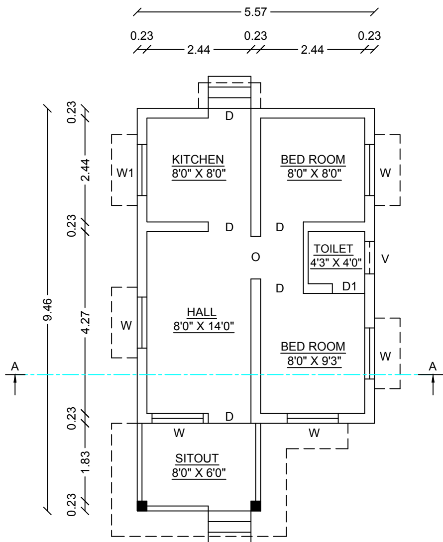
PLAN
