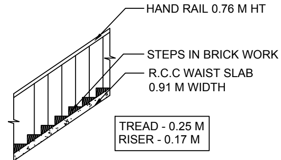
STEP DETAILS
