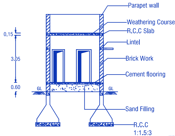
CROSS SECTION ON 'AB'
