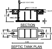
SEPTIC TANK PLAN
