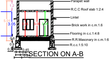
SECTION ON A-B
