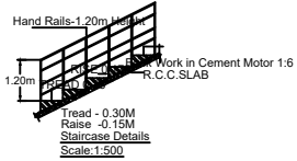
Staircases Details Scale:1:500
