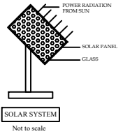
SOLAR SYSTEM Not to scale
