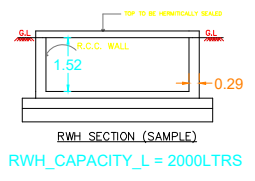
RWTH_SECTION (SAMPLE) RWTH_CAPACITY_L = 2000LTRS
