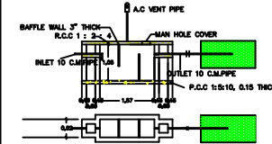
Septic Tank
