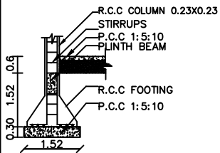
COLOUMN DETAILS
