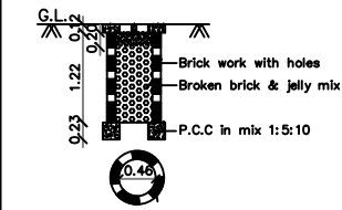
PERCOLATION PIT FOR 30 Sq. m. (Scale: - 1:50)
