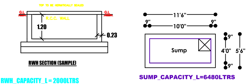
SUMP CAPACITY L=6480LTRS
