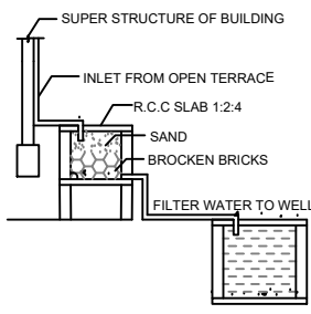
DETAILS OF FILTER BED & WELL
