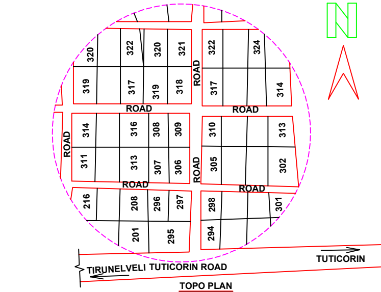
TOPO PLAN
