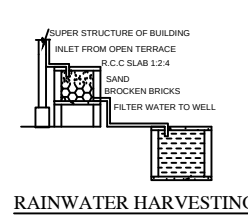
RAINWATER HARVESTING
