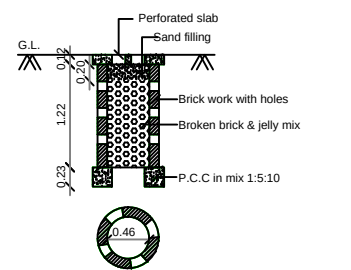
PERCOLATION PIT FOR 30 Sq. m. (Scale:- 1:50)
