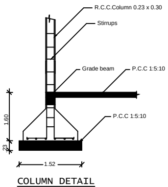
COLUMN DETAIL
