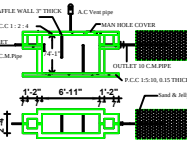
Septic tank and trench
