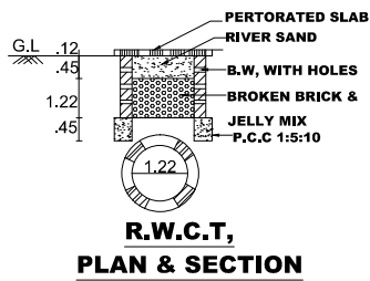
DETAILS OF COLLECTION SUMP FOR RAIN WATER HARVESTING OF ROOF TOP RAIN WATER RWV_CAPACITY_L=5000LTRS
