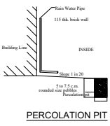
PERCOLATION PIT
