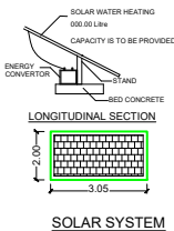
SOLAR SYSTEM
