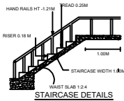
STAIRCASE DETAILS
