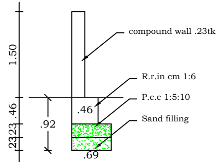
Compound wall Detail
