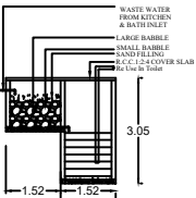
RECYCLING OF WASTE WATER FROM KITCHEN & BATHROOM
