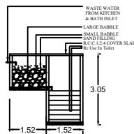
RECYCLING OF WASTE WATER FROM KITCHEN & BATHROOM
