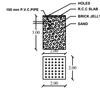
RAIN WATER COLLECTING TANK
