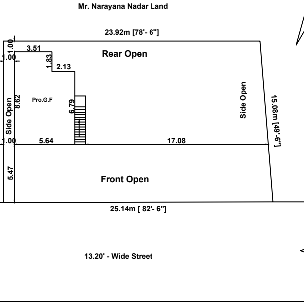
SITE PLAN
